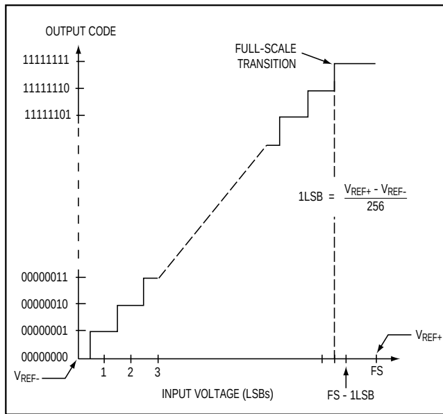
Figure 10. Transfer Function
